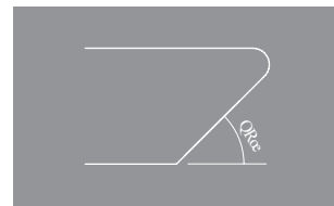
Borde redondeado a 45° Rounded ridge at 45°
